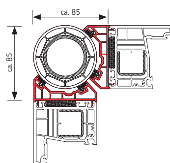
Eckverbinder variabel K 243/245
